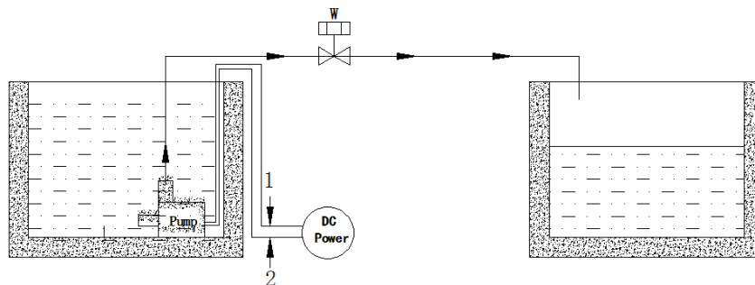
Submersible Install
