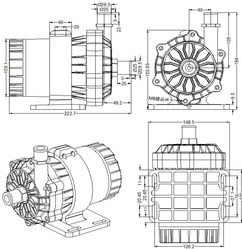
PUMP Body
